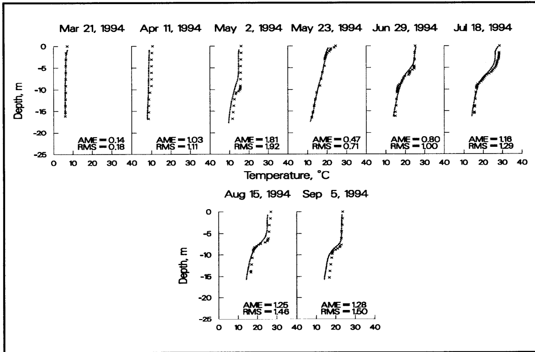
Figure 5. 1994 computed versus observed temperatures at station 1
