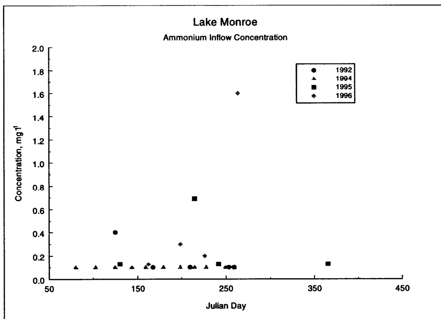
Figure A23. 1992, 1994, 1995, and 1996 inflow ammonium concentrations
