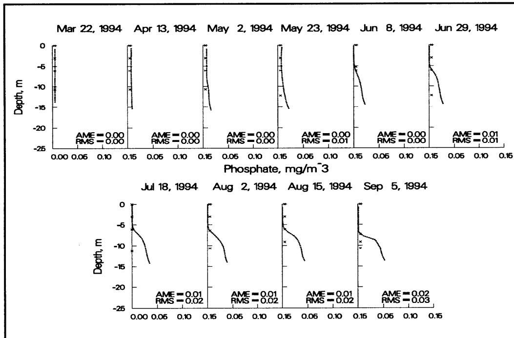
Figure 12. 1994 computed versus observed phosphorus at station 35
