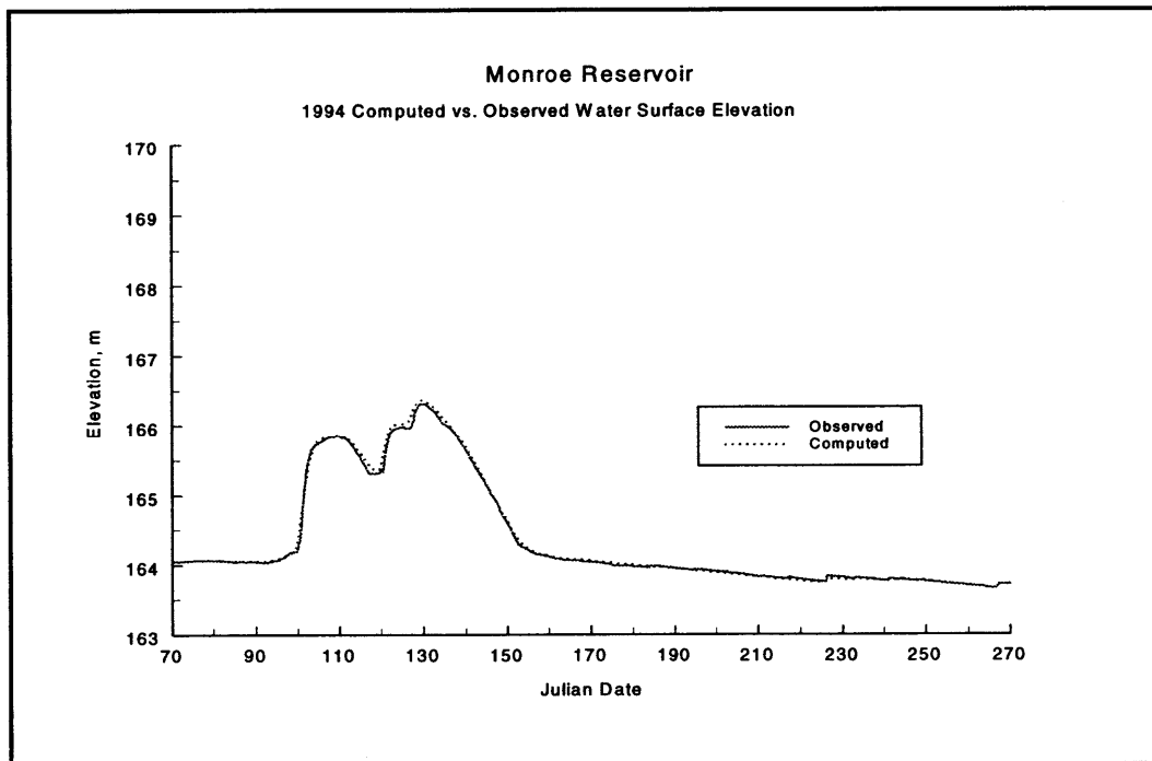
Figure 4. 1994 computed versus observed water surface elevations
