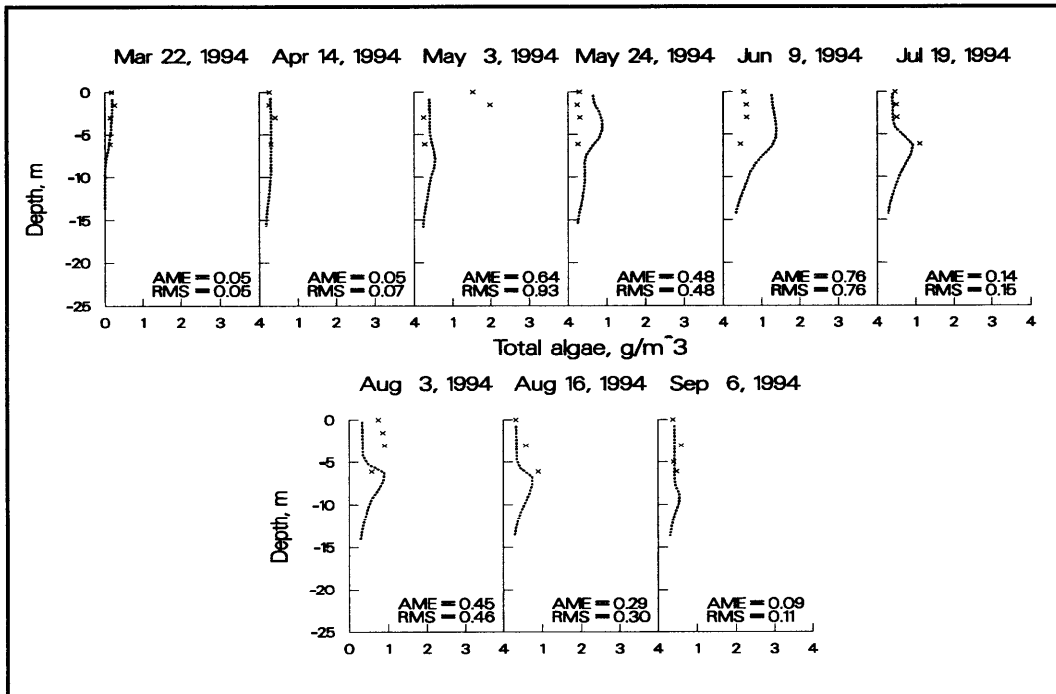
Figure 21. 1994 computed versus observed algae at station 35
