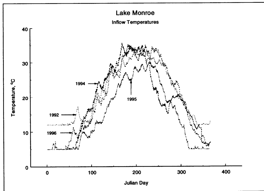
Figure A21. 1992, 1994, 1995, and 1996 inflow temperatures
