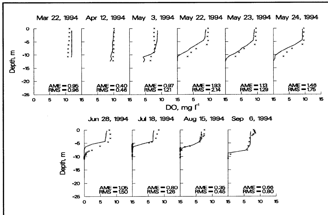
Figure 10. 1994 computed versus observed DO at station 3
