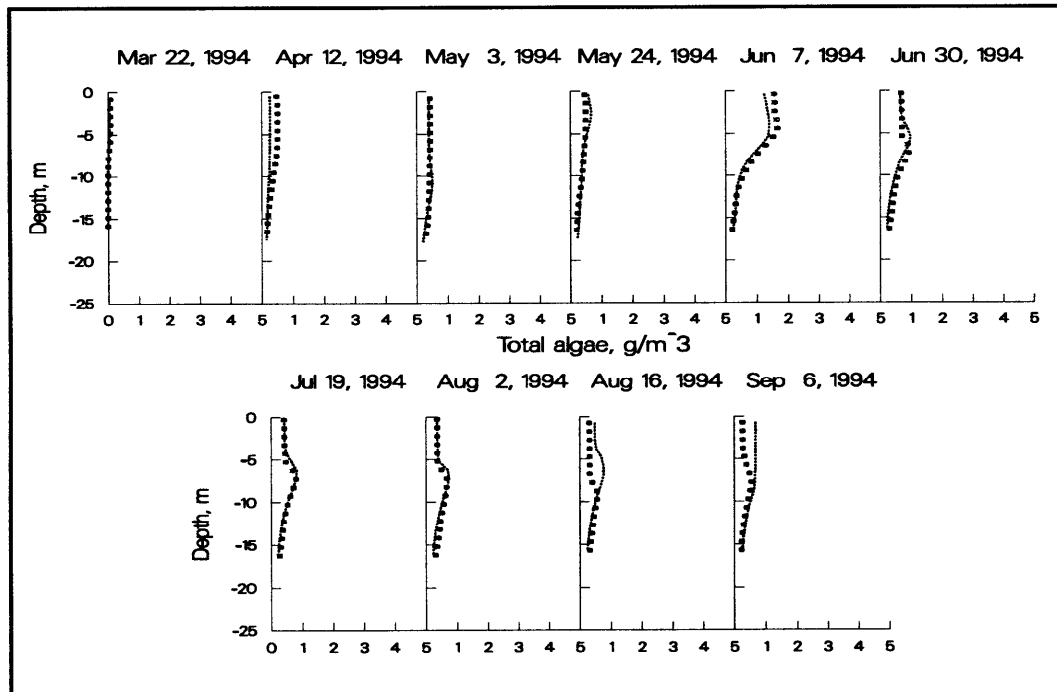
Figure 58. Algal results for base run (....), scenario 1 (xxxx) and scenario 2 (ooo)
