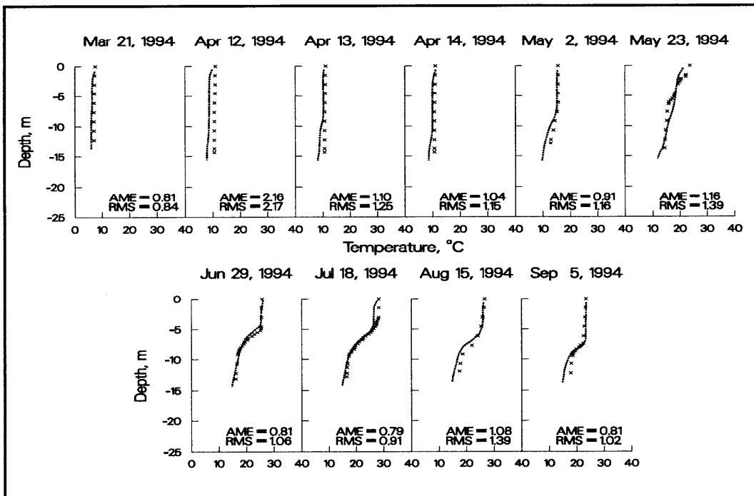
Figure 6. 1994 computed versus observed temperatures at station 35
