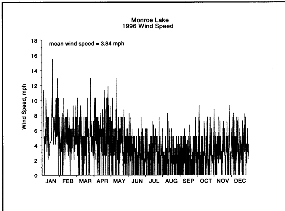
Figure A14. 1996 wind speed
