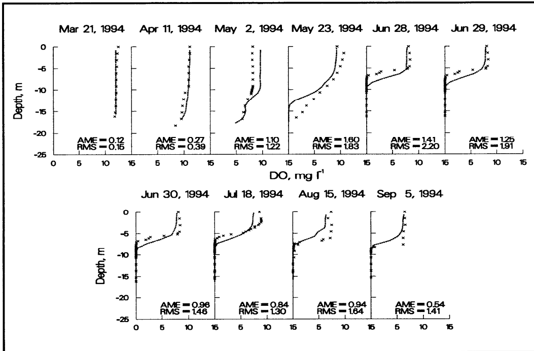
Figure 8. 1994 computed versus observed DO at station 1
