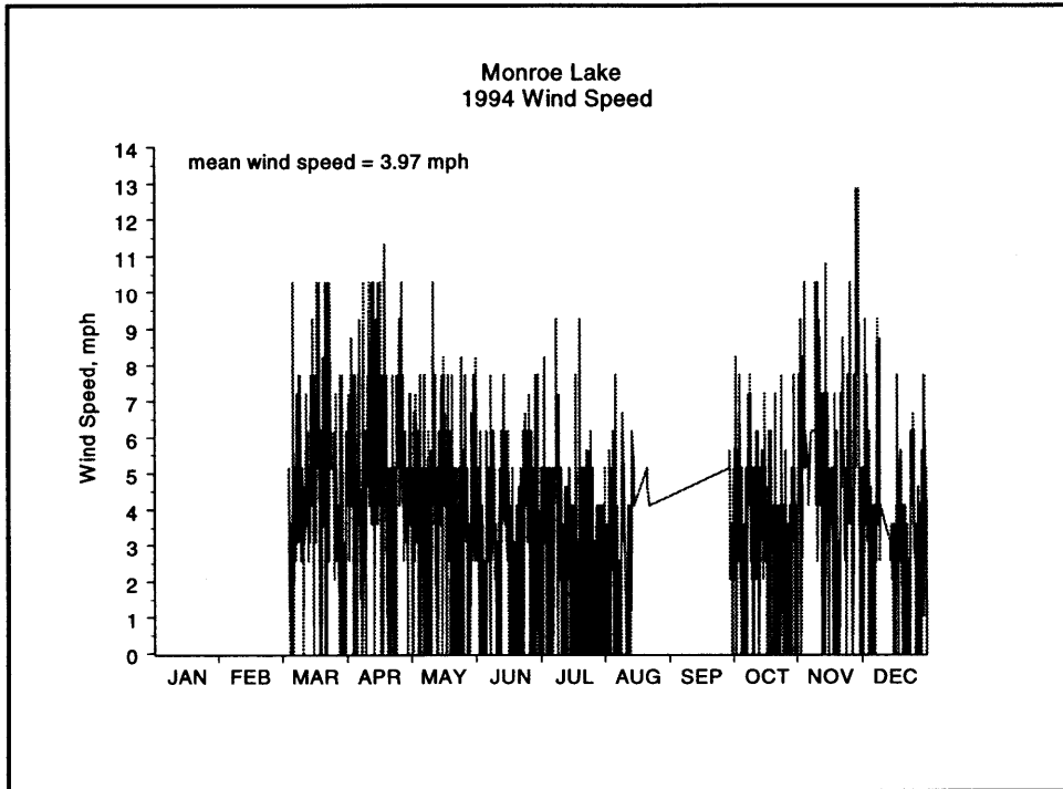
Figure A6. 1994 wind speed
