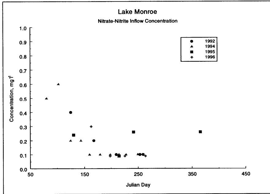
Figure A24. 1992, 1994, 1995, and 1996 inflow nitrate-nitrite concentrations
