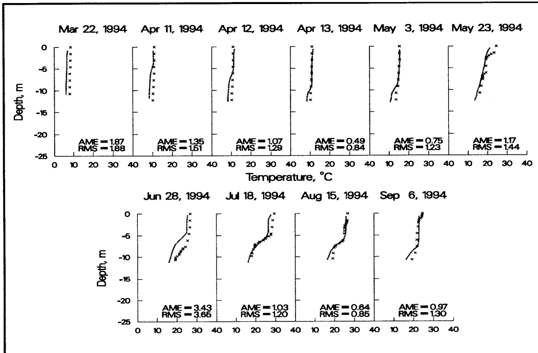
Figure 7. 1994 computed versus observed temperatures at station 3
