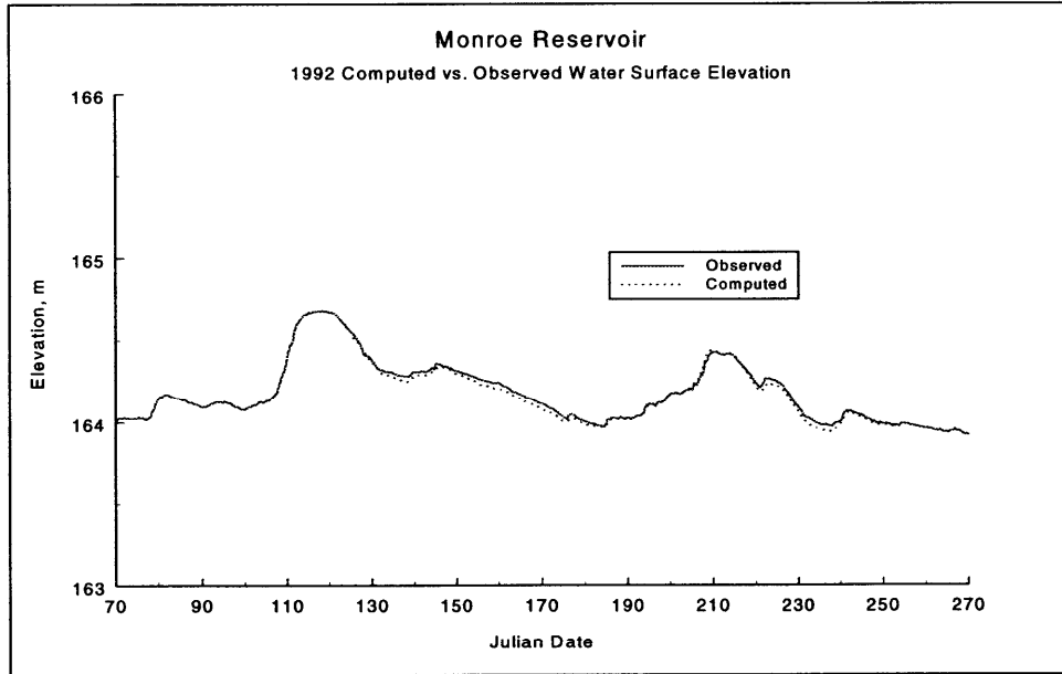
Figure 23. 1992 computed versus observed water surface elevations
