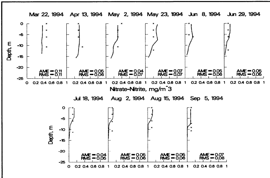
Figure 18. 1994 computed versus observed nitrate-nitrite at station 35
