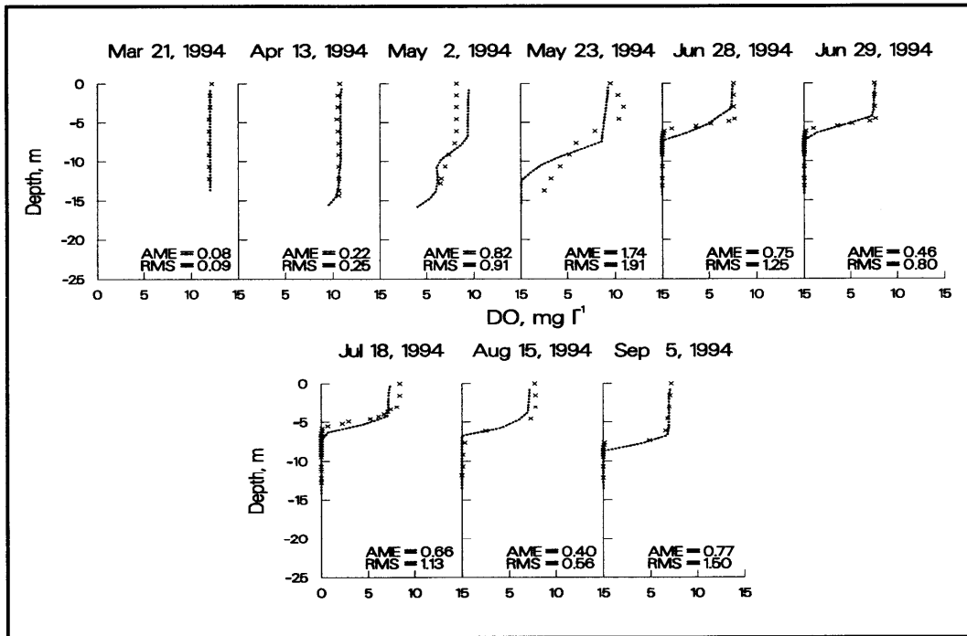
Figure 9. 1994 computed versus observed DO at station 35
