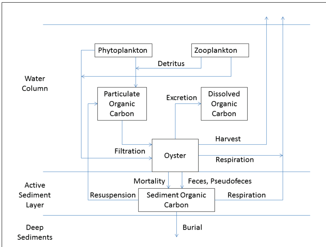
Figure 7. The model carbon cycle including oysters. The quantifiable benefits include carbon removal via fisheries harvest and carbon removal via burial to deep, inactive sediments.
