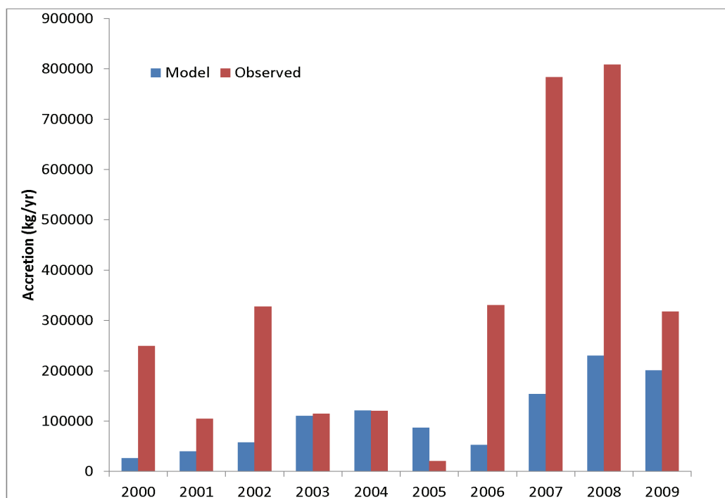
Figure 29. Computed and observed (Southworth et al. 2010) shell accretion rates.
